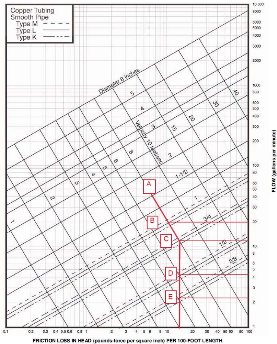
FIGURE 3-C 102.1(3) CHART A-105.4(4)-C 101.1(1) FOR FINDING PIPE SIZE
